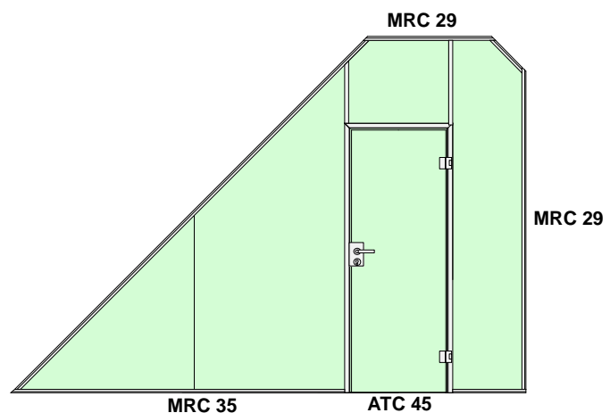
Type 550 , e.g. for roof pitches with MRC 29 and MRC 35 profiles
