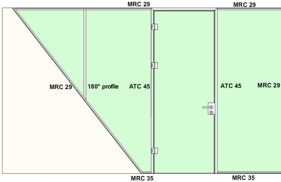
Type 660 - 29 freestanding frame with ceiling connection
