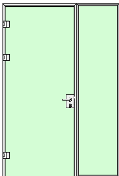
ATC 45 doorframe with glasdoor and fixed frame MRC 35
