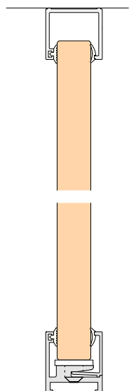
MRC 35 Frame profile
