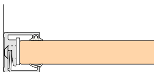
MRC 29 Frame profile for wood-fillings and plastic-boards up to 19 mm
