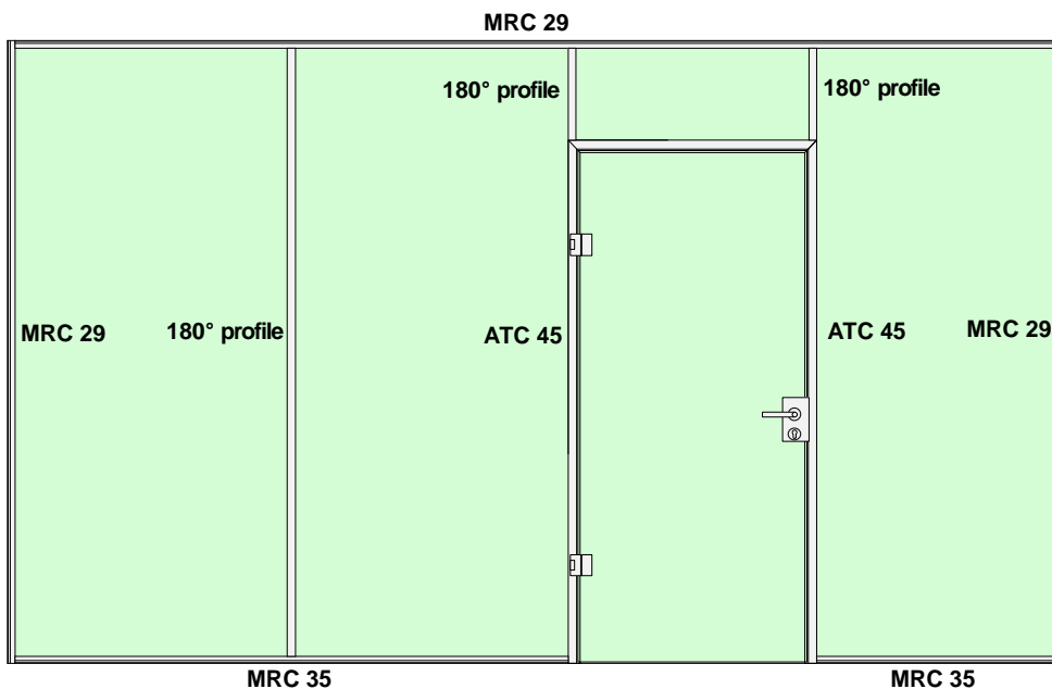
Type 650 - 29 freestanding frame with ceiling connection
