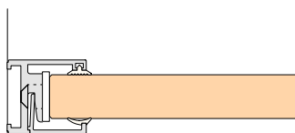
MRC 35 Frame profile for wood-fillings and plastic-boards up to 19 mm
