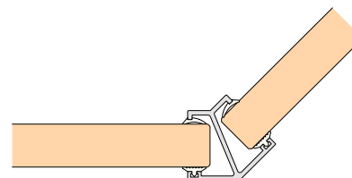
Profile No. 586 - 135°
