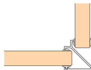
Profile No. 587 - 90°
