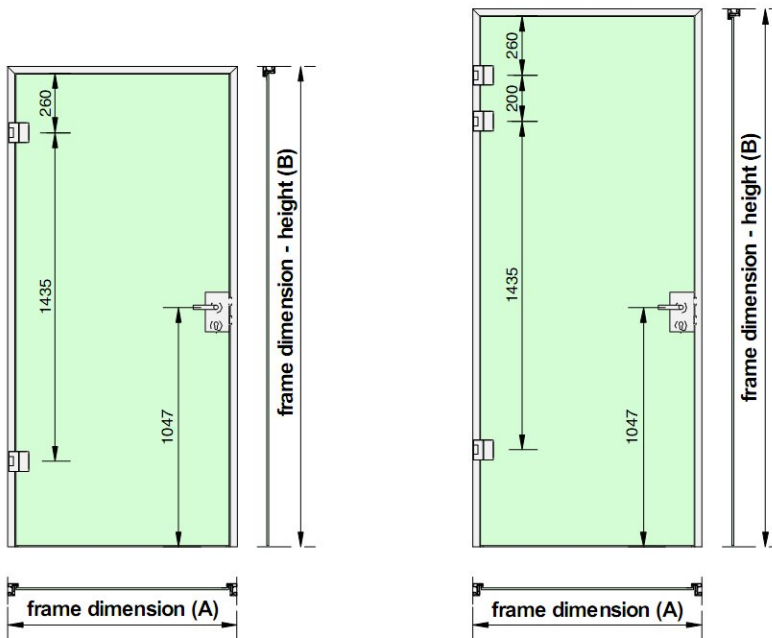
ATC 45 frame with 2 bands, lock casing + handle set
