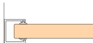
Profile No. 594 Frame profile for wood-fillings and plastic-boards up to 19 mm
